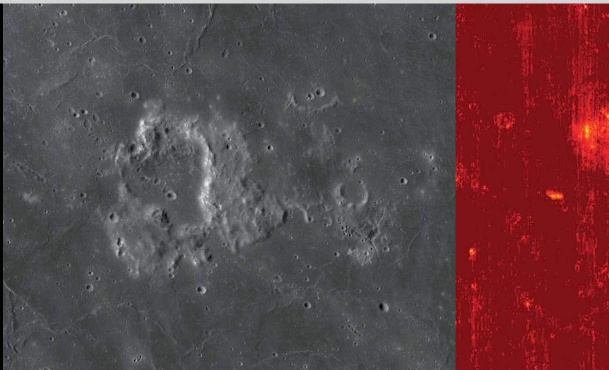
WOLF CRATER: NASA / LUNAR RECONNAISSANCE ORBITER; MID-INFRARED IMAGE: NASA / GSFC / UCLA / APL
