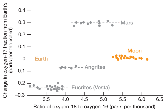
▲ OXYGEN ISOTOPES Mars, the asteroid Vesta, and angrite meteorites all have notably different ratios of oxygen's three isotopes than terrestrial samples do. Samples of the Moon, however, plot right on top of Earth's values. The x-axis spread in each population is due to chemical processing within each body.
