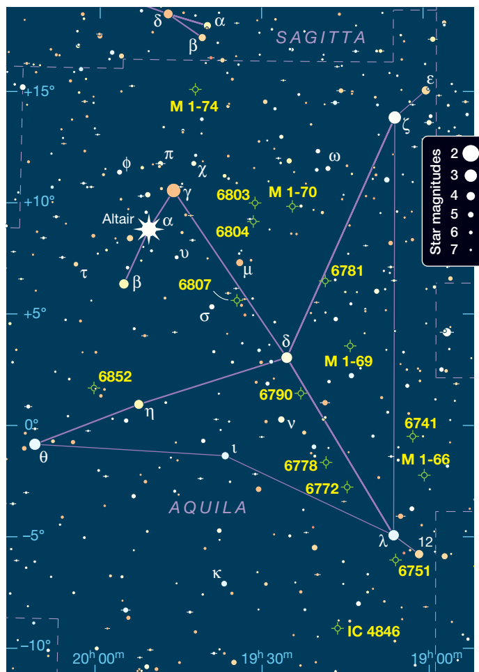
▲ SOAR WITH THE EAGLE All the targets discussed in the text except for Abell 70 (in the far southeastern corner of Aquila) appear here.
