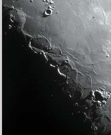
▲ Images taken under oblique solar illumination reveal Wolf (lower right) to be the southernmost feature in a chain of ruined craters.
