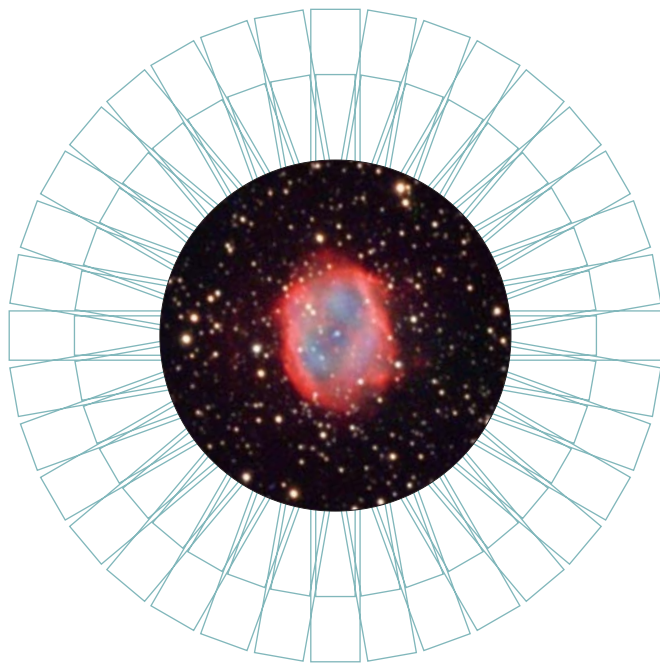
▲ ANCIENT BUBBLE OF GAS NGC 6772 is an evolved planetary nebula with a rather low surface brightness. Dark, transparent nights are recommended for trying to spot this diffuse annulus.
