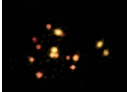
▲ ALMA imaged 14 galaxies swarming like fireflies in a massive protocluster that existed 1.4 billion years after the Big Bang.
