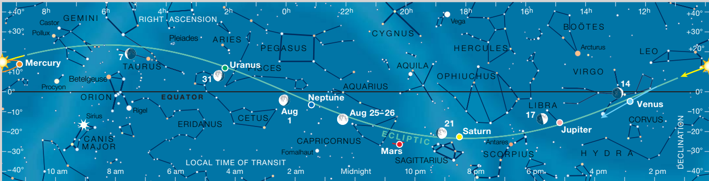
The Sun and planets are positioned for mid-August; the colored arrows show the motion of each during the month. The Moon is plotted for evening dates in the Americas when it's waxing (right side illuminated) or full, and for morning dates when it's waning (left side). "Local time of transit" tells when (in Local Mean Time) objects cross the meridian — that is, when they appear due south and at their highest — at mid-month. Transits occur an hour later on the 1st, and an hour earlier at month's end.
