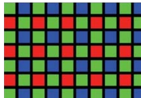
BAYER MATRIX Color cameras have monochrome detectors with a microscopic grid — known as a Bayer matrix — of red, green, or blue filters placed over each pixel. This information is then re-interpreted as the color image.
